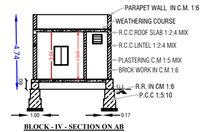
BLOCK - IV - SECTION ON AB
