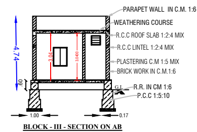
BLOCK - III - SECTION ON AB
