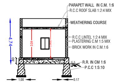
BLOCK - II - SECTION ON AB
