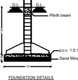
FOUNDATION DETAILS
