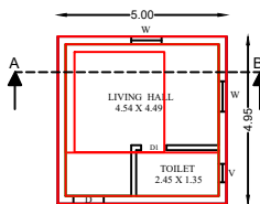
BLOCK - II GROUND FLOOR
