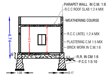
BLOCK - I - SECTION ON AB
