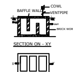
SEPTIC TANK DETAILS NOT TO SCALE
