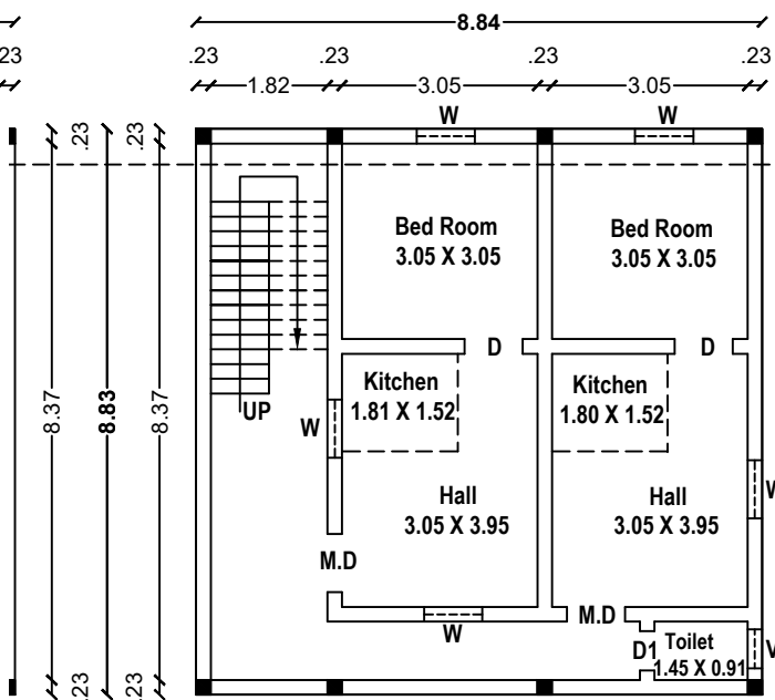
Residential First Floor Plan
