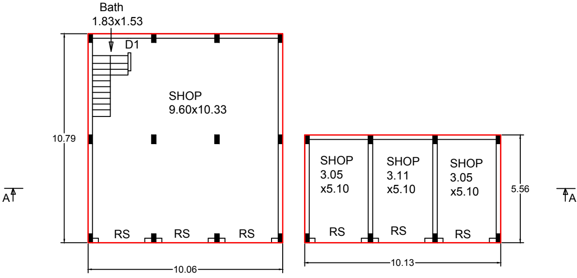
PLAN - Ground Floor
