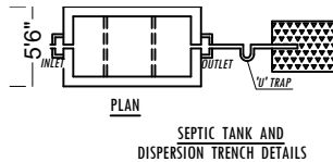
SEPTIC TANK AND DISPERSION TRENCH DETAILS
