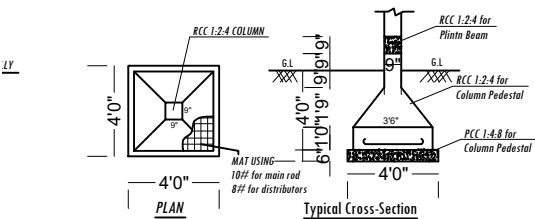
FOOTING DETAILS
