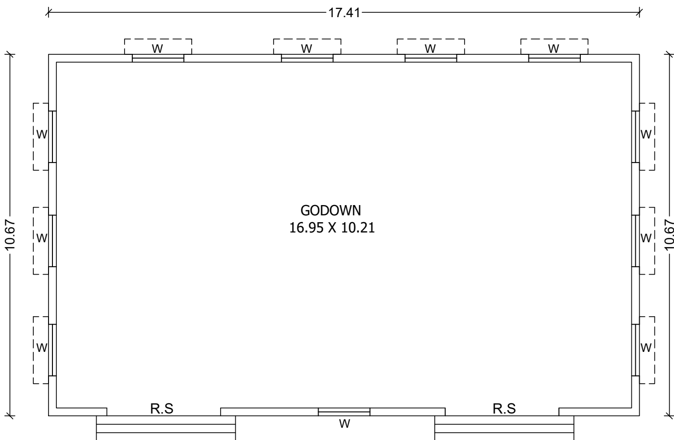
GROUND FLOOR PLAN NORTH FACING
