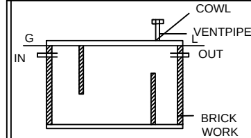
SECTION ON - XY
