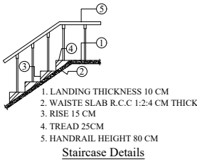
Staircase Details
