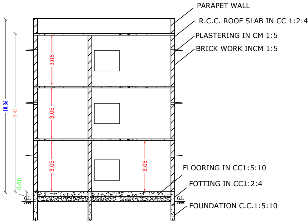
SECTION ON "AAAA"
