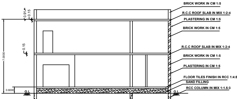
SECTION-ON AB
