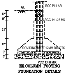
EX.COLUMN FOOTING FOUNDATION DETAILS
