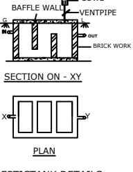
SEPTICTANK DETAILS
