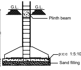
FOUNDATION DETAILS
