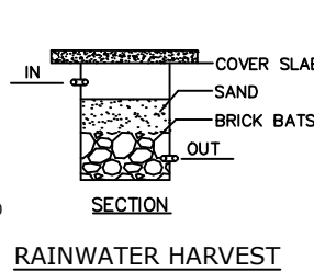
RAINWATER HARVEST
