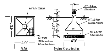
FOOTING DETAILS
