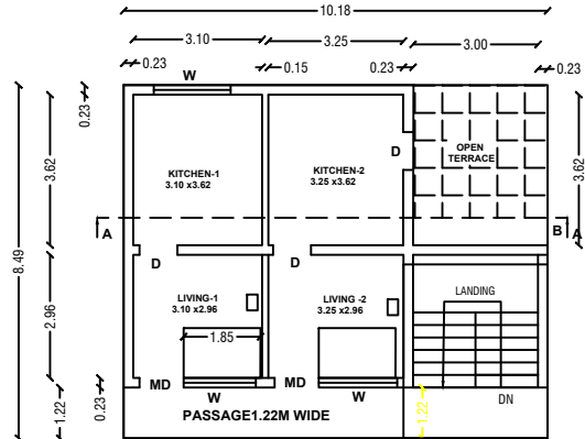
FIRST FLOOR PLAN (Residential)
