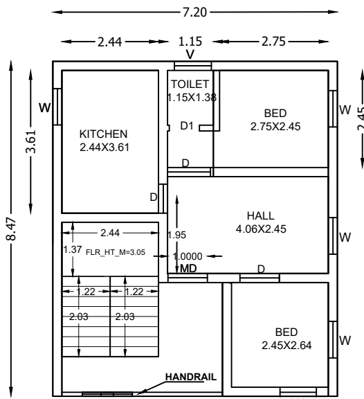
PROPOSED SECOND FLOOR
