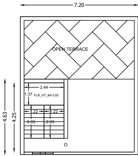
PROPOSED HEAD ROOM TERRACE FLOOR
