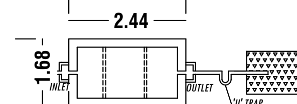
PLAN SEPTIC TANK AND DISPERSION TRENCH DETAIL
