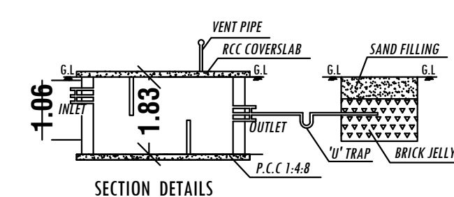
SECTION DETAILS
