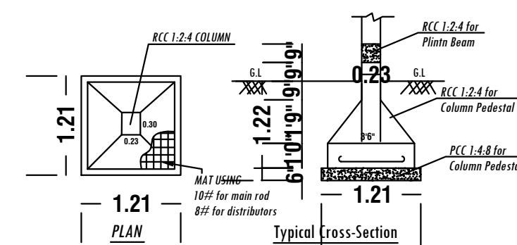
FOOTING DETAILS
