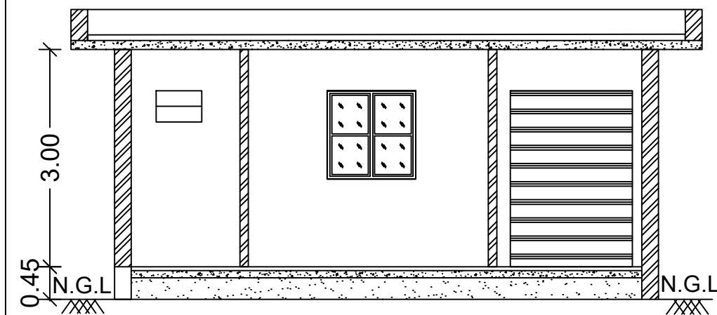
SECTION ON-"AB"
