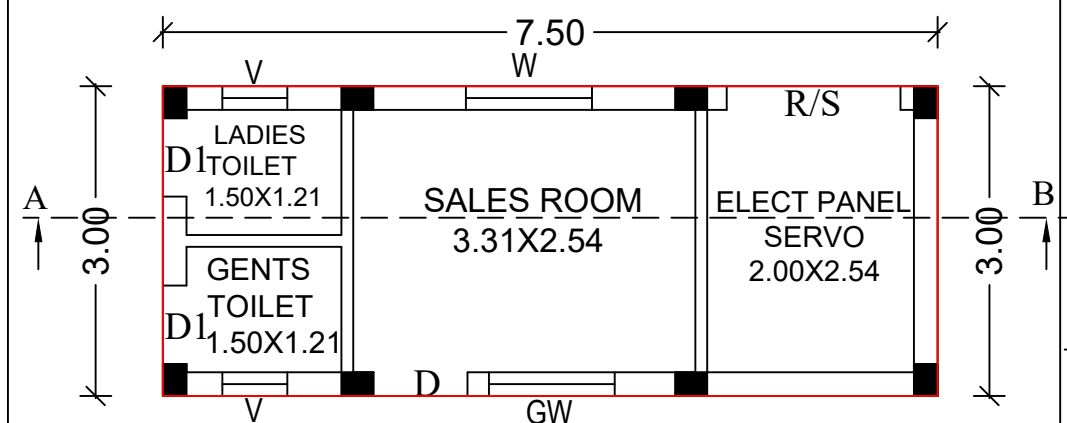
GROUND FLOOR PLAN SALES BLOCK
