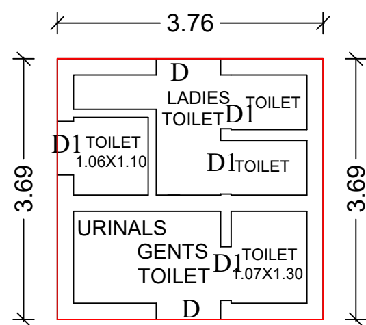
TOILET GROUND FLOOR PLAN
