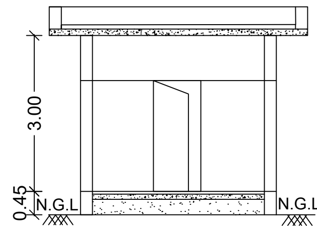
SECTION ON-"CD"
