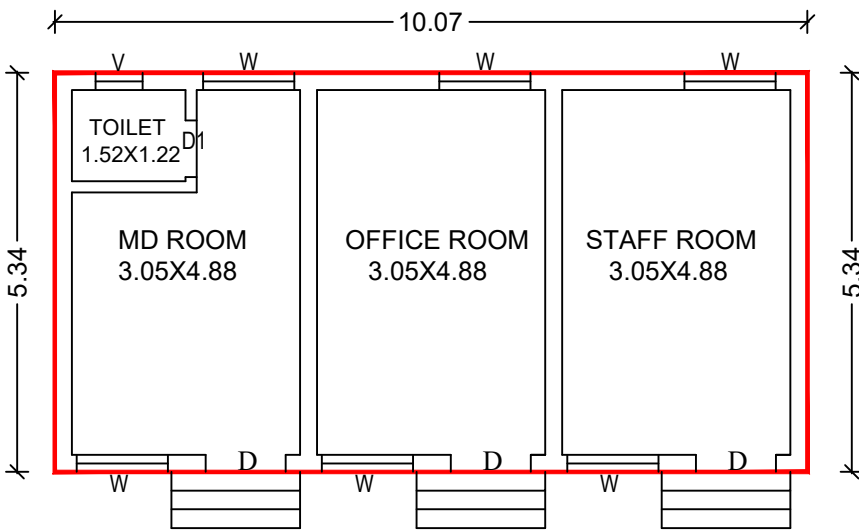
GROUND FLOOR PLAN OFFICE BLOCK
