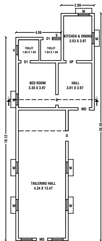
RESIDENTIAL & COMMERCIAL GROUND FLOOR PLAN
