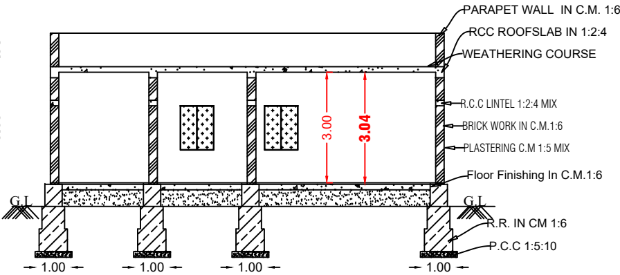
SECTION ON-"AB"
