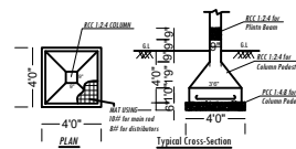
FOOTING DETAILS
