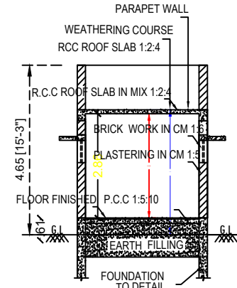
SECTION "A-B"
