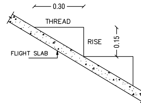
STAIRCASE DETAILS
