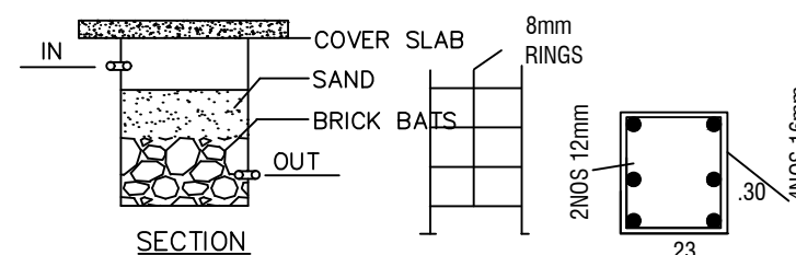
COLUMN DETAILS (NOT TO SCALE)
