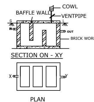
SEPTICTANK DETAILS NOT TO SCALE
