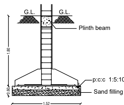
FOUNDATION DETAILS
