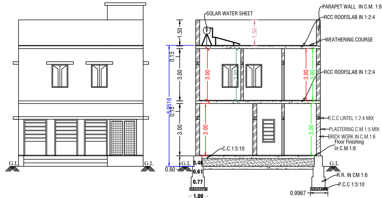
Front Elevation
