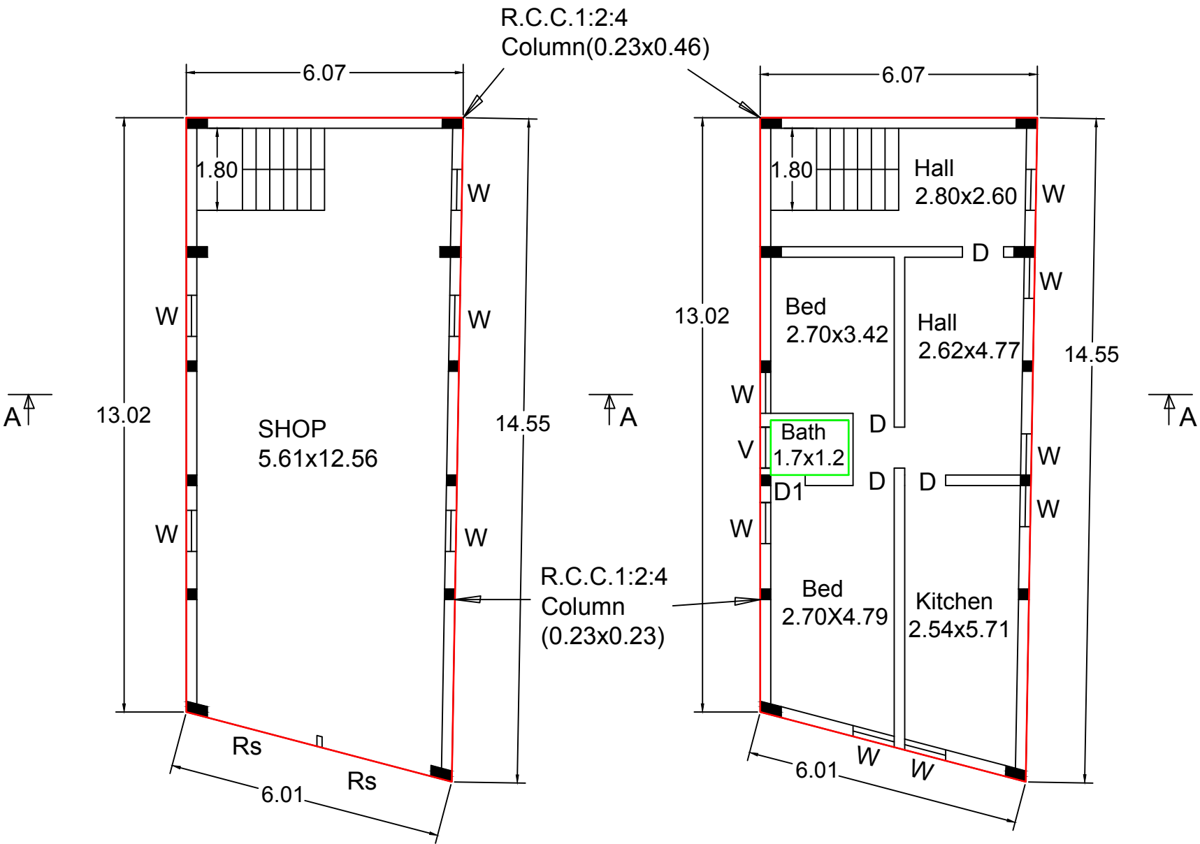
Plan - First Floor (House)
