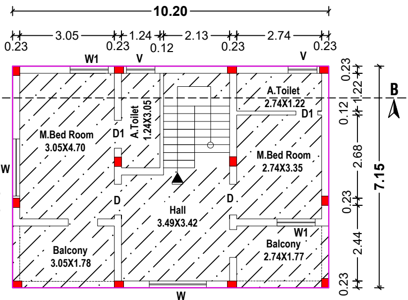
Ext.First Floor Plan
