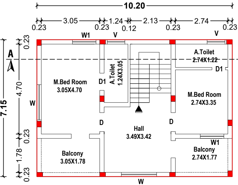
Pro.Second Floor Plan
