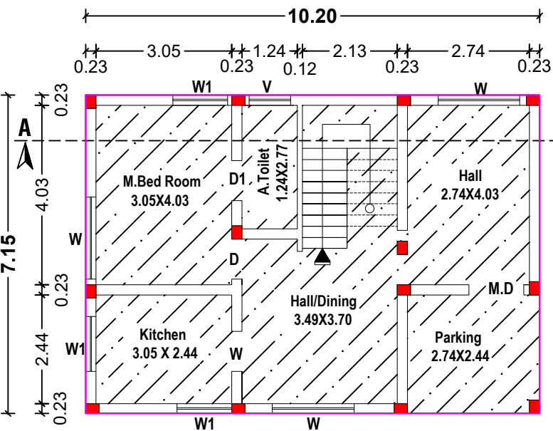
Ext.Ground Floor Plan
