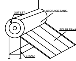
SOLAR SYSTEM
