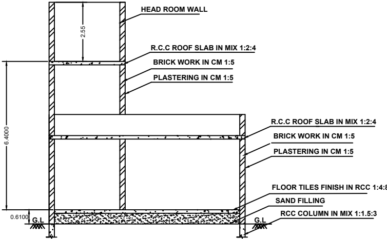
SECTION-AB
