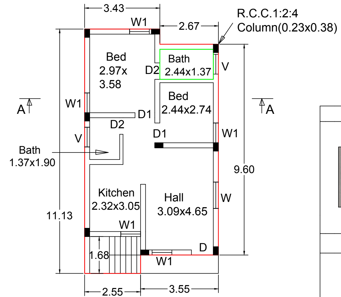
PLAN
