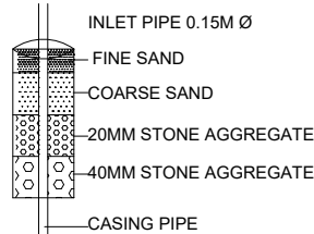
DETAILS OF RAIN WATER HARVESTING STRUCTURES
