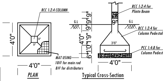
FOOTING DETAILS
