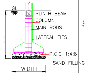
FOUNDATION DETAILS
