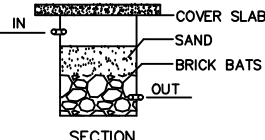
SECTION
