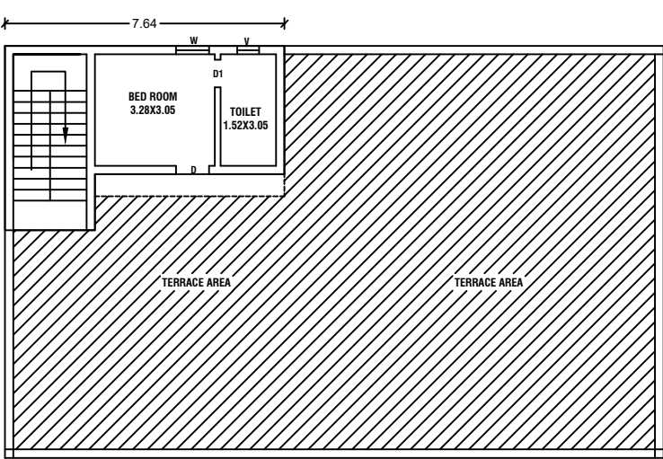
SECOND & TERRACE FLOOR PLAN
