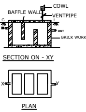
SEPTICTANK DETAILS
