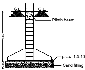
FOUNDATION DETAILS
