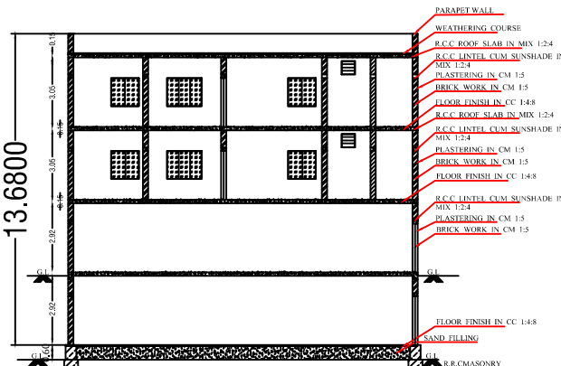
SECTION ON-'AB'
