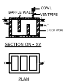
SEPTICTANK DETAILS (NOT TO SCALE)
