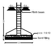
FOUNDATION DETAILS
