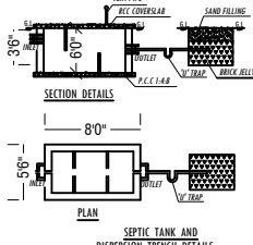
SECTION DETAILS
