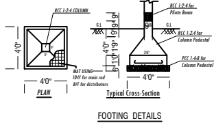
FOOTING DETAILS
