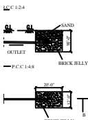
FOUNDATION DETAILS (SCALE 1:100)
