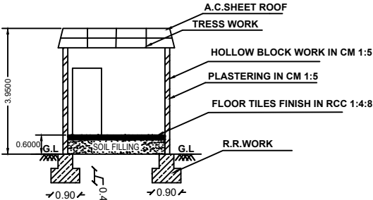
SECTION-AB
