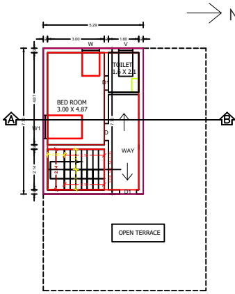
RISE 0.15 TREAD 0.25 RCC1: 2; 4 WAIST SLAB 0.15 THICK
