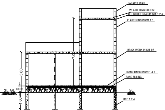
SECTION ON "MA"
