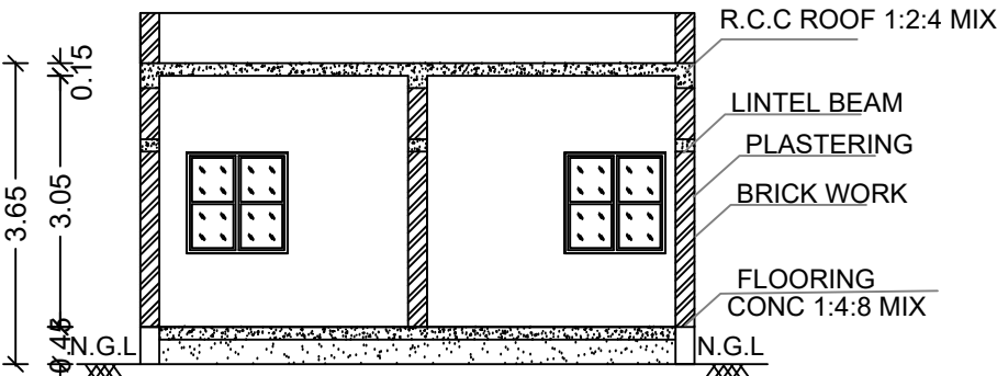
SECTION ON-"AB"
