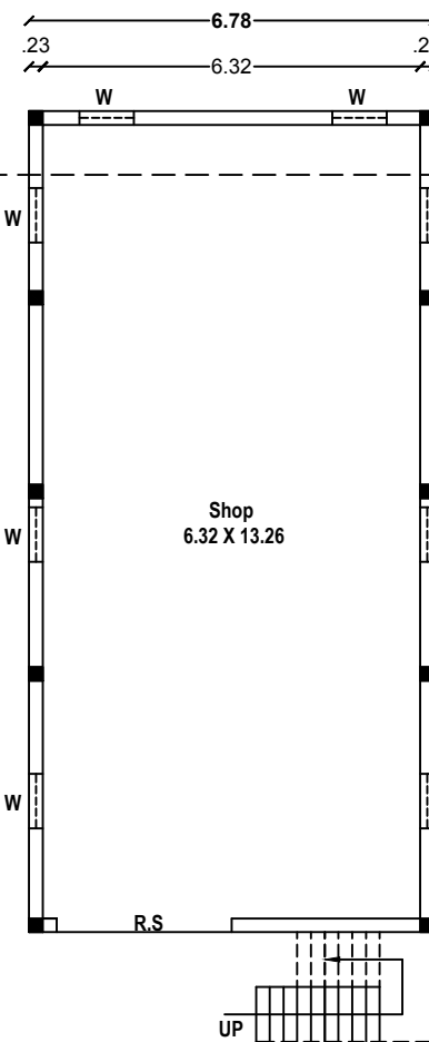
Exi - Commercial Ground Floor Plan
