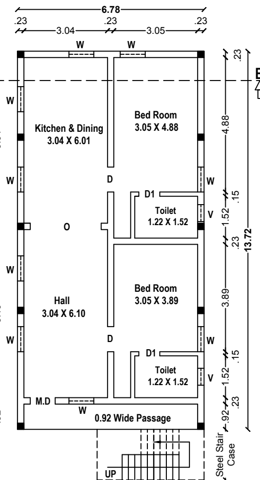
Pro - Residential First Floor Plan
