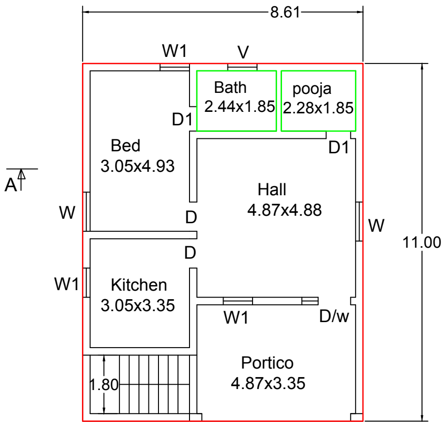
PLAN - GROUND FLOOR
