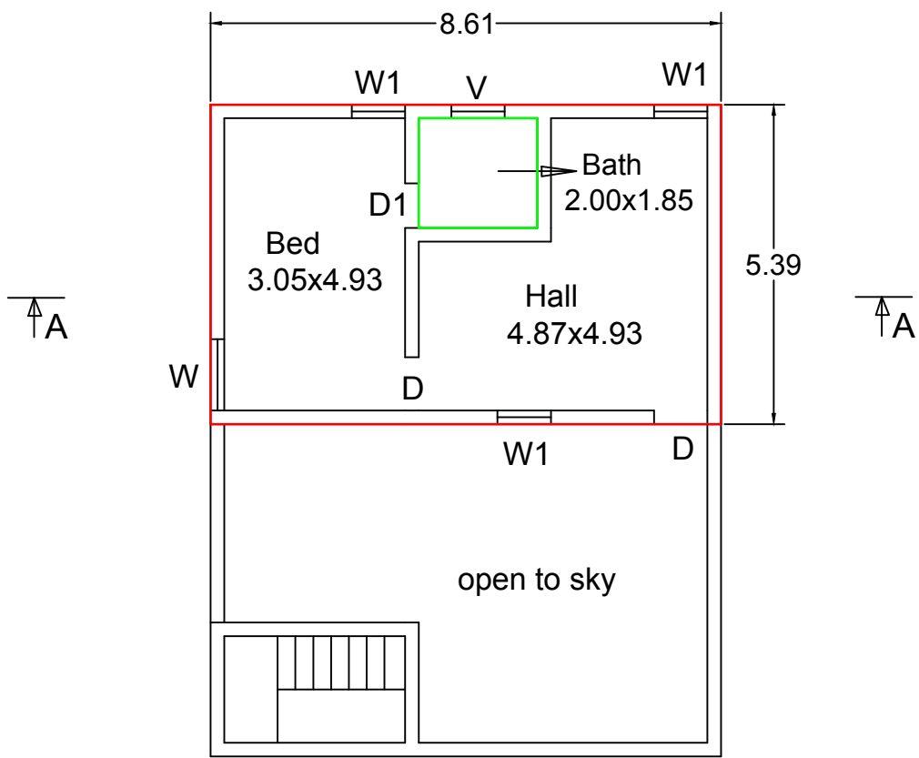
PLAN - FIRST FLOOR
