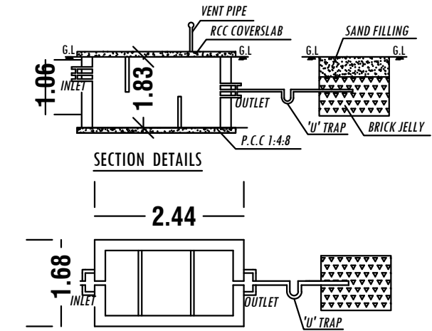
SEPTIC TANK AND DISPERSION TRENCH DETAILS
