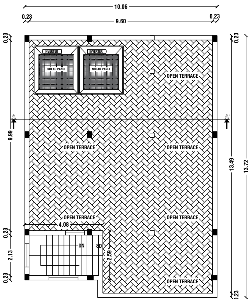
HEAD ROOM CUM OPEN TERRACE FLOOR PLAN
