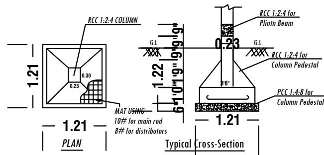
FOOTING DETAILS
