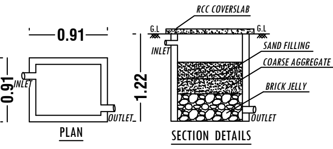
RAINWATER HARVESTING SYSTEM
