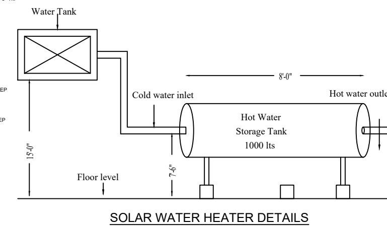
SOLAR WATER HEATER DETAILS
