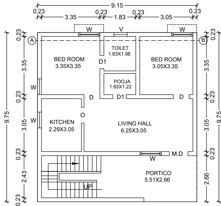
GROUND FLOOR PLAN EAST FACING
