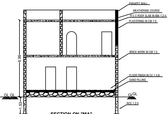
SECTION ON "MA"
