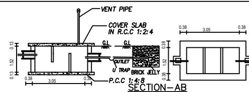
SEPTIC TANK & DISPERSION TRENCH SCALE DETAIL 1100
