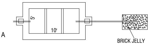
SEPTIC TANK & DISPERSION TRENCH DETAILS
