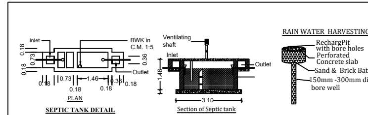
SEPTIC TANK DETAIL
