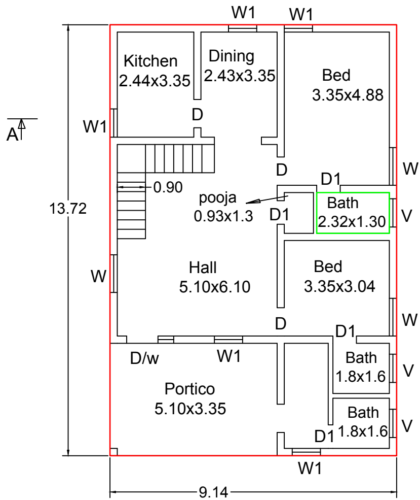
PLAN - GROUND FLOOR
