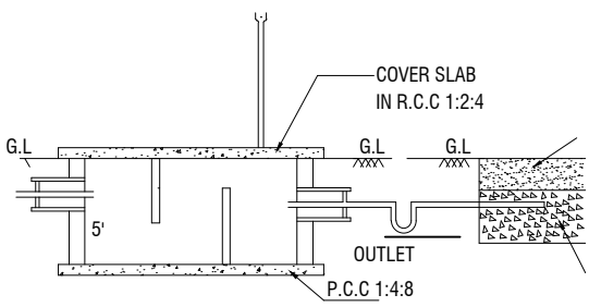
SECTION-AB
