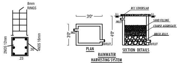
COLUMN DETAILS (NOT TO SCALE)
