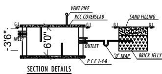
SECTION DETAILS
