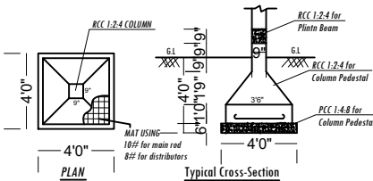
FOOTING DETAILS
