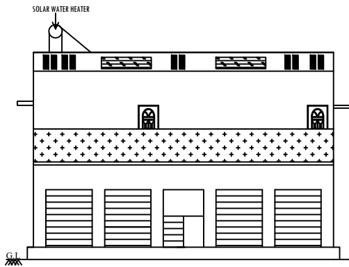
ELEVATION PLAN
