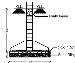
FOUNDATION DETAILS
