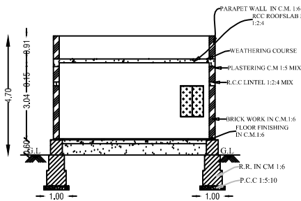
SECTION ON-"AB"
