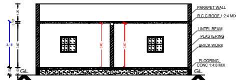
SECTION : "A-B"
